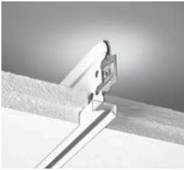
Stab-End 4600 System Cross Tee Non-Fire Rated
