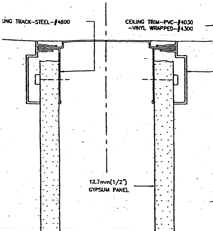
1. HEAD DETAIL
