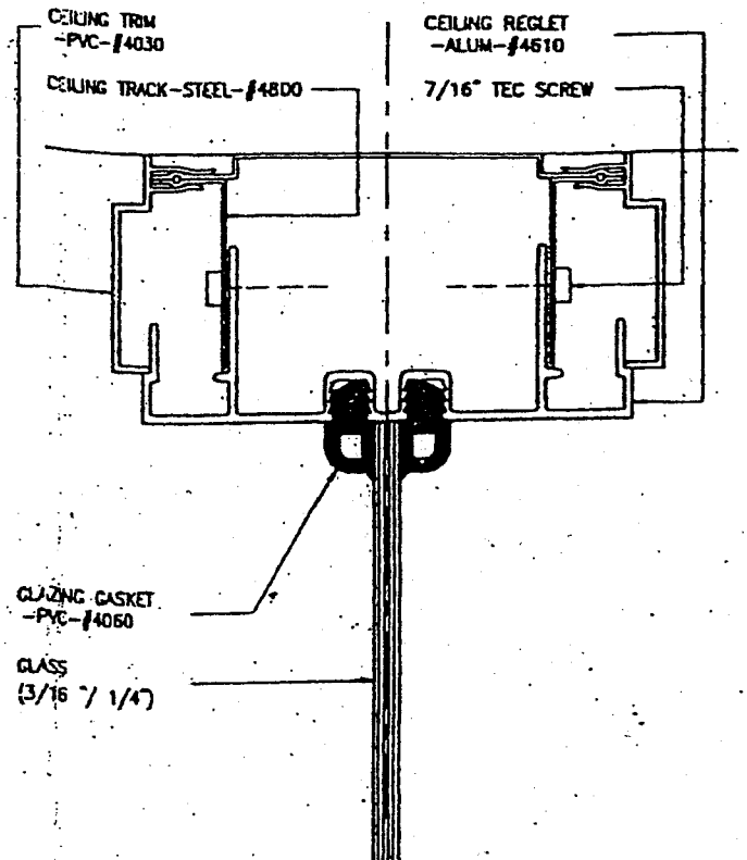
2. CEILING HEIGHT GLAZING HEAD
