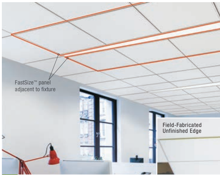
Ultima® Beveled Tegalur 24" x 24" and 22" x 24" FastSize™ panels with Silhouette® 1/4" reveal 9/16" suspension system (pg. 395) and 4" linear light fixtures
